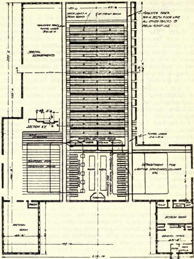
FIG. 123—FIRST FLOOR PLAN, PLANT NO. 10
